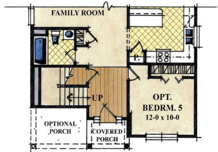
OPTIONAL BEDROOM 5 W/ALT. FIRST FLOOR PLAN
